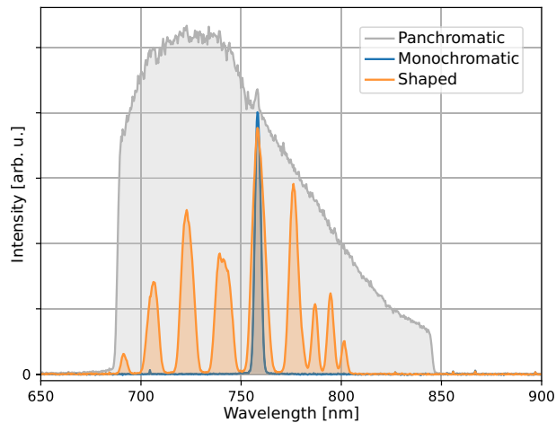
Fig. 5. The three illumination spectra generated with S^3 : panchromatic spectrum (gray), monochromatic spectrum offering maximum contrast between AlOx and AlGaAs (blue), shaped spectrum (orange) corresponding to all the bands with positive contrast (see fig. 4(c)).
