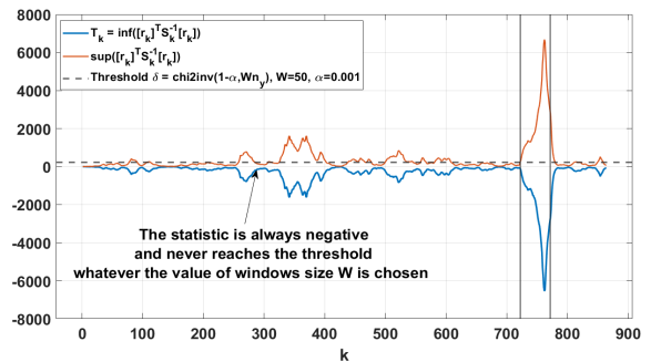
Fig. 4. Method A - Fault detection using statistic T_k = \text{inf}([r_k]^T \mathcal{S}_k^{-1} [r_k]) for Bicycle model.
