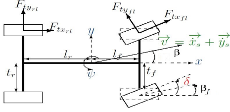
Fig. 2. View of the bicycle model reproducing the lateral behaviour of the car.
