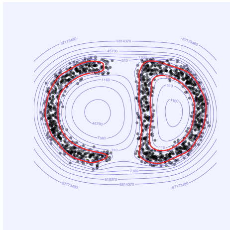
FIGURE 2. Level sets \mathcal{S}_\gamma associated with \Lambda_{10}^{\phi_N} for various values of \gamma ; the red level set is obtained with \gamma := s(10) ; reprinted from cover of [15, p. 45] with permission. ©Cambridge University Press
