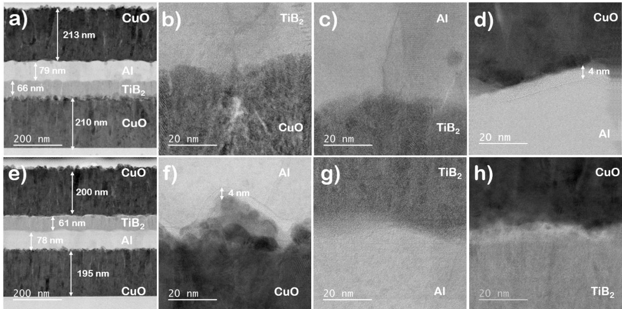
Figure 3: STEM images showing as deposited multilayers and the corresponding interfaces: a) CuO-TiB 2 -Al-CuO b) CuO-TiB 2 c) TiB 2 -Al d) Al-CuO and e) CuO-Al-TiB 2 -CuO f) CuO-Al g) Al-TiB 2 h) TiB 2 -CuO. All interfaces are observed to be quite dense with no delamination.
