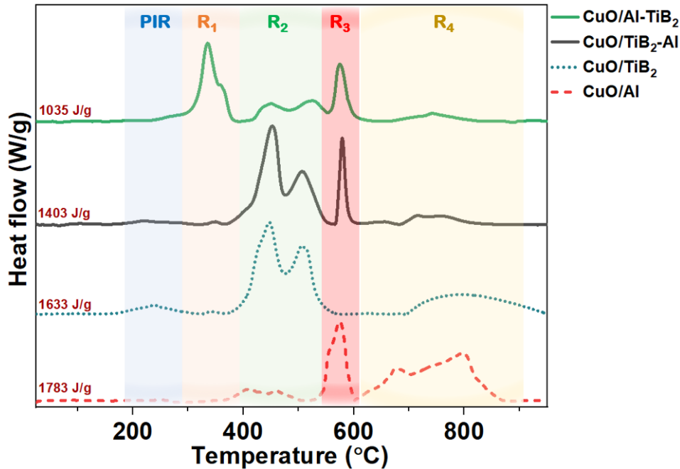
Figure 2: DSC traces of 5 BL CuO/Me {Me: Al, TiB 2 , TiB 2 -Al}. The traces are baseline subtracted manually and are offset in Y to provide clarity. The plot is divided into 5 regions: a pre-ignition region (PIR), regions R 1 , R 2 , R 3 and R 4
