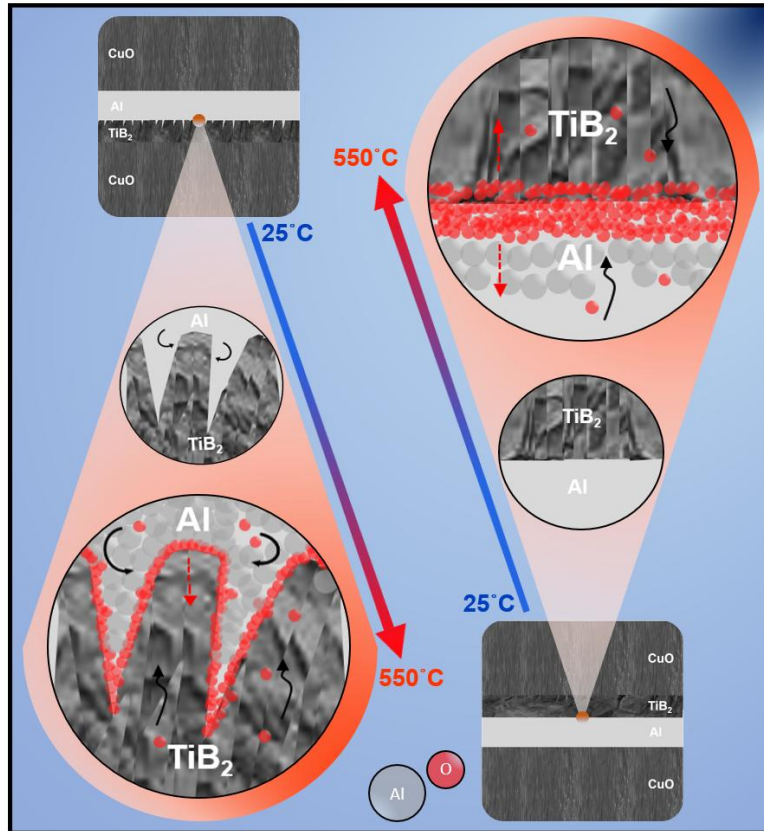
Figure 5: Schematic of an outlook on the oxidation and potential microstructural changes of \text{TiB}_2\text{-Al} and \text{Al-TiB}_2 interfaces. While the oxide layer (in red) can grow bidirectionally in \text{CuO-Al-TiB}_2\text{-CuO} , \text{CuO-TiB}_2\text{-Al-CuO} features a unidirectional oxide growth which is inhibited by Al due to lower probability of \text{Al-O} bond formation than that of \text{Ti-O}
