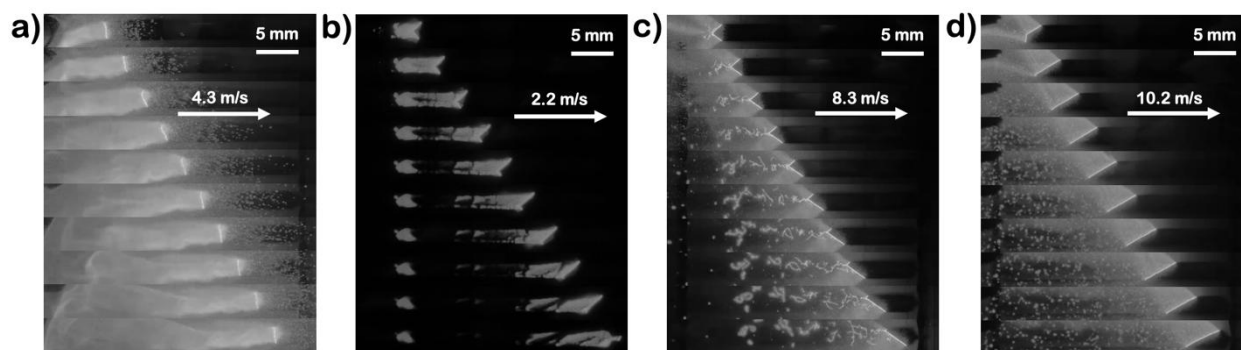
Figure 1: Snapshots from propagation of 5 BL CuO/Me {Me: a ) Al, b ) TiB 2 , c ) TiB 2 -Al and d ) Al-TiB 2 }
