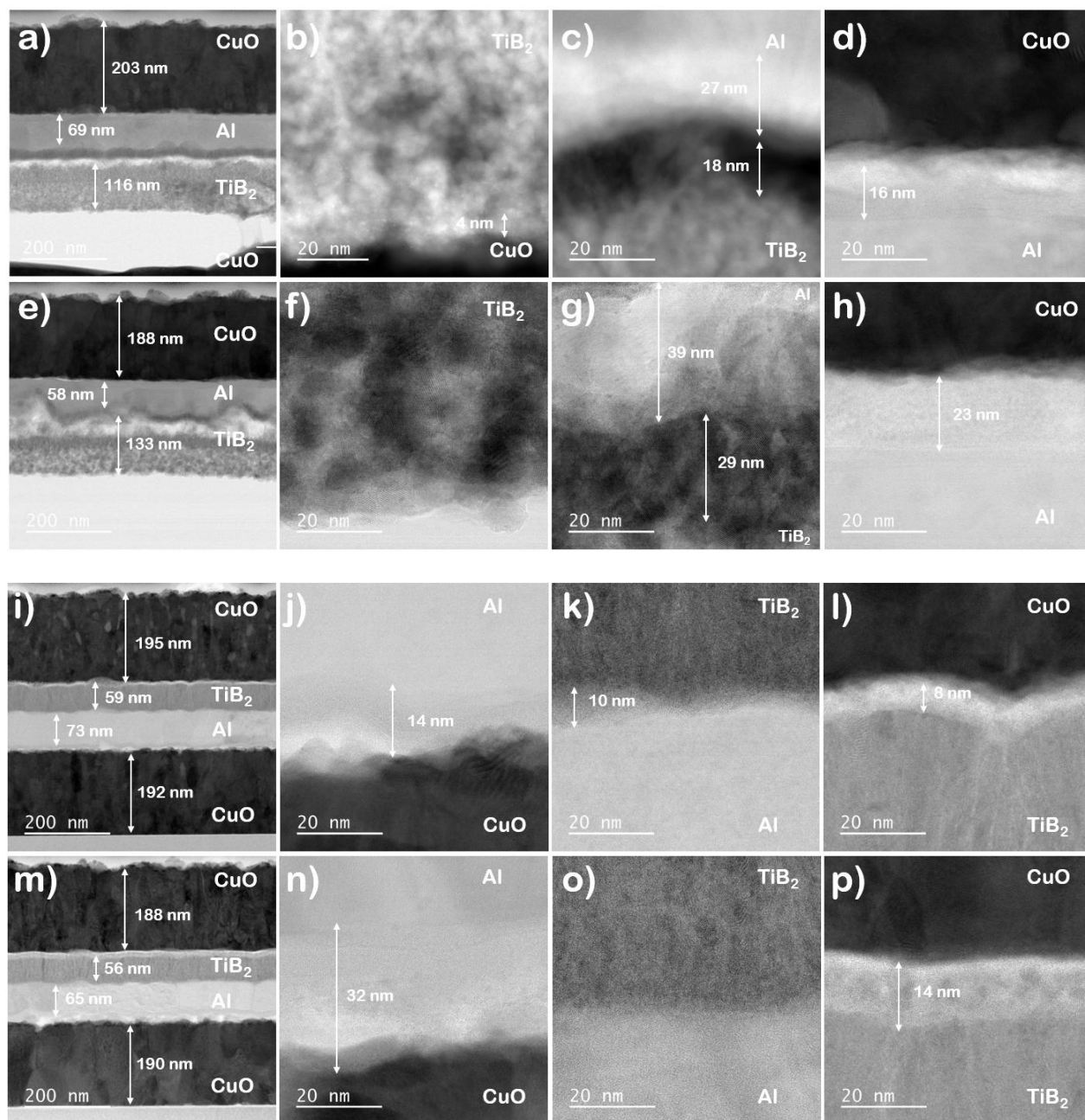
Figure 4: STEM images showing annealed multilayers and the corresponding interfaces: a) CuO-TiB 2 -Al-CuO annealed at 475 °C and its interfaces ( b-d ), e) CuO-TiB 2 -Al-CuO annealed at 550 °C and its interfaces ( f-h ), i) CuO-Al-TiB 2 -CuO annealed at 375 °C and its interfaces ( j-l ), m) CuO-Al-TiB 2 -CuO annealed at 480 °C and its interfaces ( n-p )
