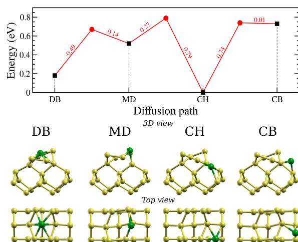
Figure 3: Energy diagram of the atomic diffusions of one Ni atom adsorbed on the Si(100) surface. Activation barriers (numerical values in red) are given in eV. 3D side and top views of each atomic configuration are provided.
