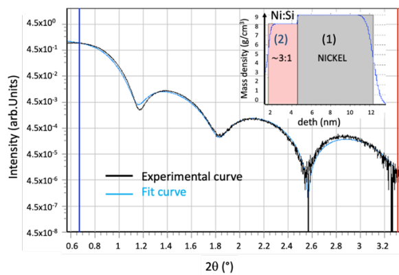
Figure 7: XRR profile of the as deposited sample. A schematic of the layered structure and obtained composition is provided in the inset: red area reveals a Ni:Si with a composition of 3:1. The blue curve represents the fit arising from the model which is in good agreement with the experimental data.
