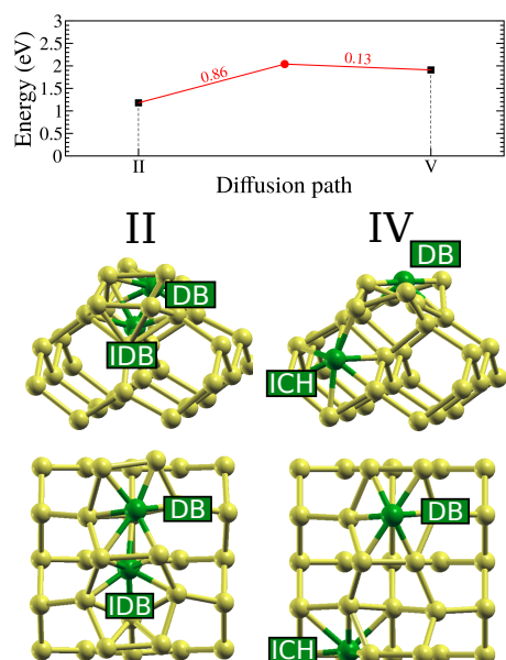
Appendix B. An additional explored path of the diffusion of two Ni atoms between an IDB+DB structure and an ICH+DB structure. This explored path indicates that it is not favorable for the Ni atom to diffuse far from the topmost layer at this level of coverage. Activation barriers (numerical values in red) are given in eV.
