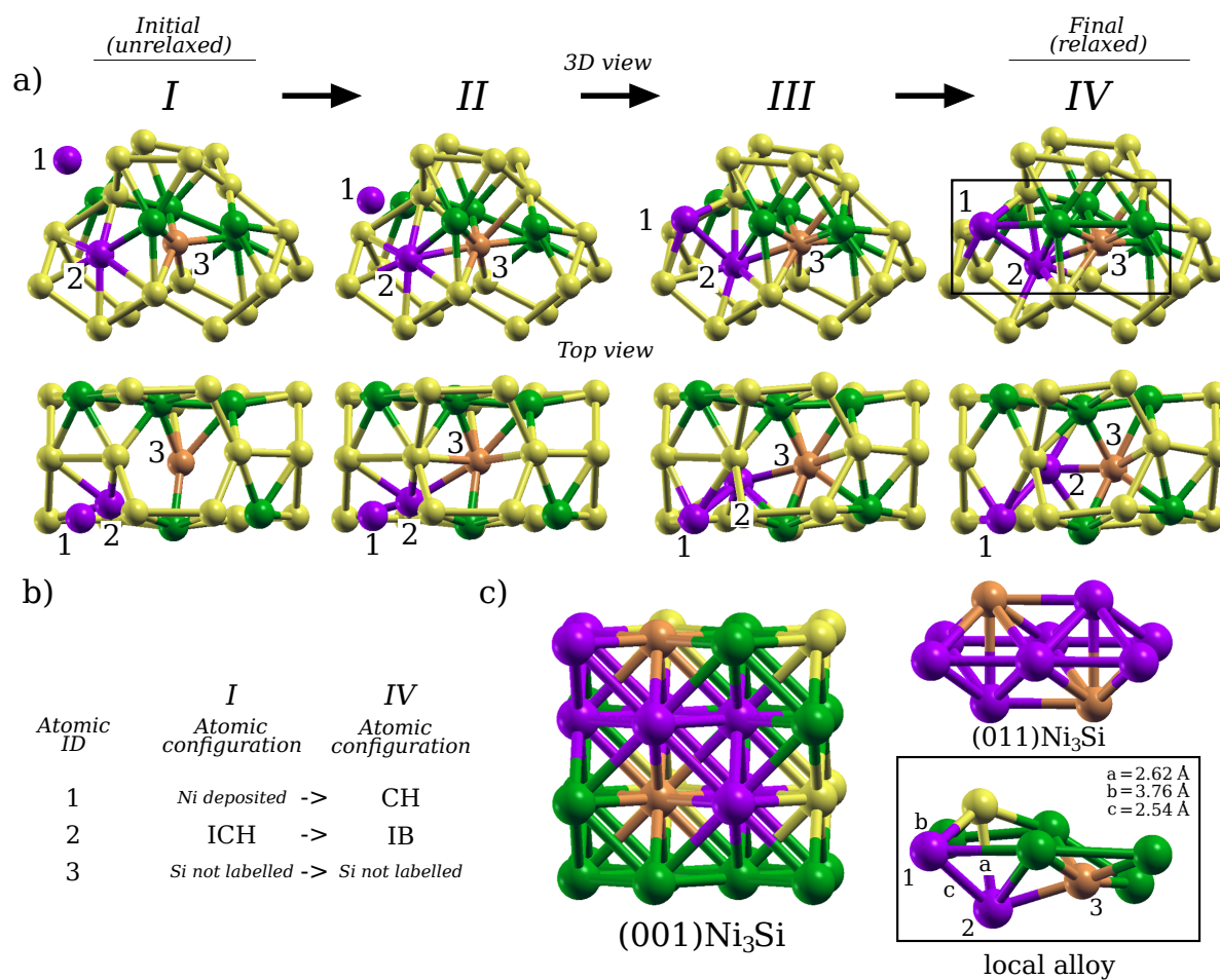
Figure 6: Formation of a Ni:Si alloyed layer with 3:1 composition. a) Adsorption of the tenth Ni atom. The starting configuration contains nine Ni atoms already adsorbed: three in IDB and six in ICH (not all shown for readability – see Appendix C). The tenth deposition site is indicated by the position 1 in snapshot I. Snapshot IV shows the relaxed configuration after the tenth adsorption. The purple atom labelled 1 is the adsorbed nickel atom. The purple Nickel atom labelled 2 and the orange silicon atom labelled 3 are the displaced atoms changing local configurations upon adsorption. The frame in snapshot IV referred to frame in c). b) Adopted configurations of atoms 1, 2, 3 highlighted in a) from snapshots I and IV in a). c) Local silicide formed: unit cell of Ni 3 Si is provided where the local alloy is highlighted using orange and purple colors. The correspondence with the local alloy is highlighted on the right with the help of the analysis on the distances altogether with an atomic positioning. Green and purple spheres are nickel atoms and yellow and orange spheres are silicon atoms. Purple and orange are used to highlight atom movements.
