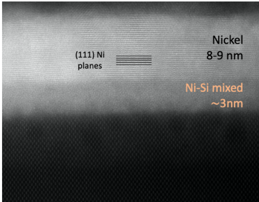
Figure 8: HR-STEM cross-section of the as deposited sample. An amorphous Ni-Si mixed layer of 3nm is clearly visible in between the brighter unreacted nickel layer on top and the dark silicon substrate at the bottom.
