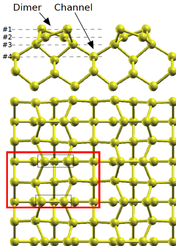
Figure 2: (top) Side view and (bottom) top view of the Si(001) surface with dimers rows separated by channels, and the indexed four topmost layers. Red rectangle: region of the surface for the Ni deposition considering the surface symmetries. Black rectangles: positions of the dimers inside the red rectangle.
