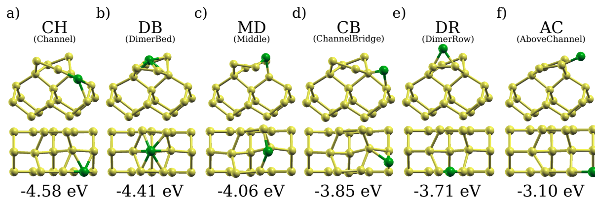
Appendix A. Stable adsorption sites of Ni on the Si (001) surface with their corresponding adsorption energies E_{ads} . Yellow and green spheres represent Si and Ni atoms, respectively.
