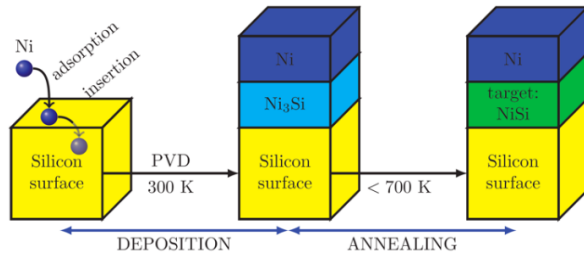
Figure 1: Schematic representation of the different stages needed to obtain NiSi silicide. The deposition of Ni atoms is first deposited with Physical Vapor Deposition (PVD) at ambient temperature forming an as-deposited interface of Ni 3 Si composition, which is then annealed at temperature below 700 K to form the targeted NiSi layer.
