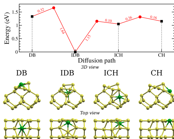
Figure 4: Insertion paths from DB (from left to right) and CH (from right to left) configurations into the topmost layers of the silicon substrate. The resulting configurations are labeled IDB (InsertedDimerBed) and ICH (InsertedChannel) 3D side and top views of each atomic configuration are provided. Activation barriers (numerical values in red) are given in eV.
