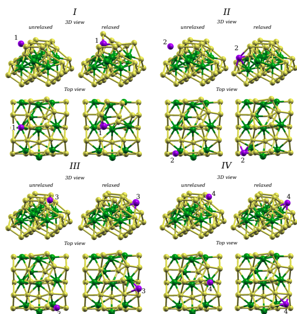
Appendix C. Adsorption of the eleventh Ni atom on the relaxed structure shown in Figure 6. Four configurations are shown. Added Ni atoms is shown as a purple sphere.
