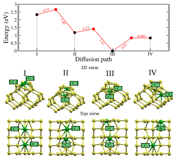
Figure 5: Most favorable insertion paths of two Ni atoms initially situated in DB configurations (from left to right) and insertion path of two Ni atoms initially situated in IDB + CH configuration (from right to left). Activation barriers (numerical values in red) are given in eV. An additional explored path is given in Appendix B.
