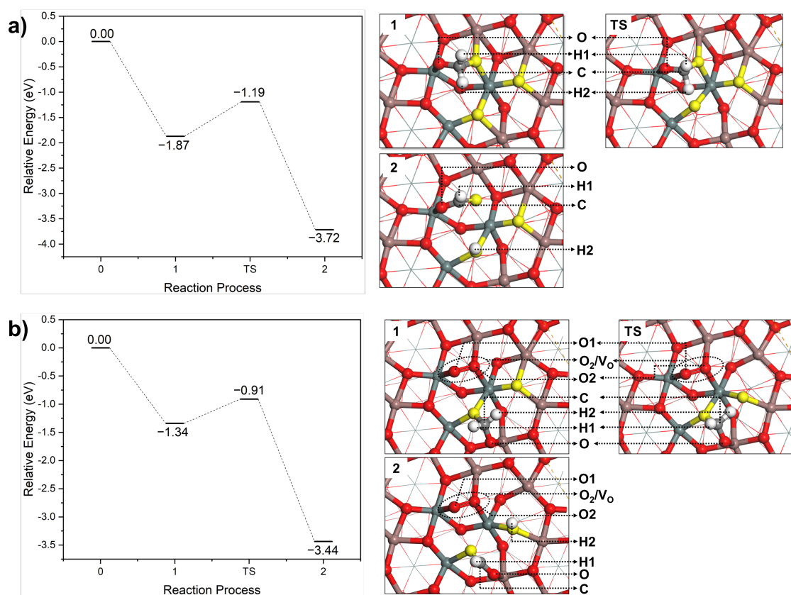
Figure 3 HCHO adsorption and oxidation at: (a) Stoichiometric In 4 Sn 3 O 12 (001) and (b) In 4 Sn 3 O 12 (001) O 2 /V O (● H, ● C, ● O, ● In, ● Sn; the bright yellow atom ● is the active O; TS means transition state.)
