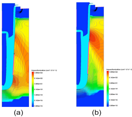
Fig. 6: Impact ionization view and electric field lines of SG-MOSFET at breakdown. Pink line shows the position of positive charges used in BV_{dss} simulations: (a) electric field with two hot spots in virgin structure; (b) for degraded structure, the high ionization spot is located in the upper portion of the trench, causing the BV_{dss} drop due to FP effect loss.
