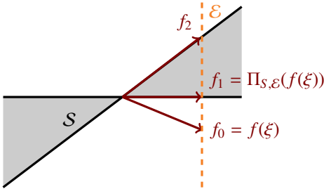
Fig. 1: Depiction of a counterexample showing that K_F(\xi) \cap T_S(\xi) \neq \Pi_{S,\mathcal{E}}(\xi, f(\xi)) , for \xi \in K \cap -K . In particular, K_F(\xi) = \text{co}\{f_0, f_2\} and K_F(\xi) \cap T_S(\xi) = \text{co}\{f_1, f_2\} \neq \{f_1\} .
