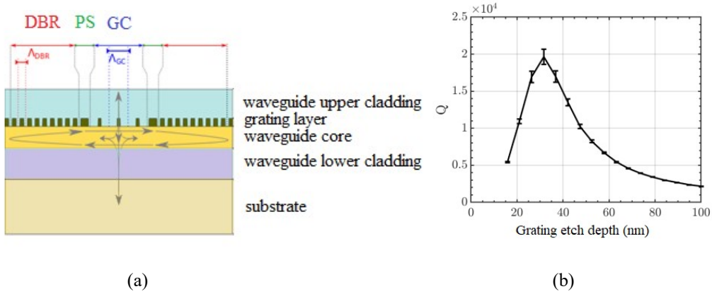
Figure 1. (a) Schematic of conventional CRIGFs where the arrows indicate how the device operates.
