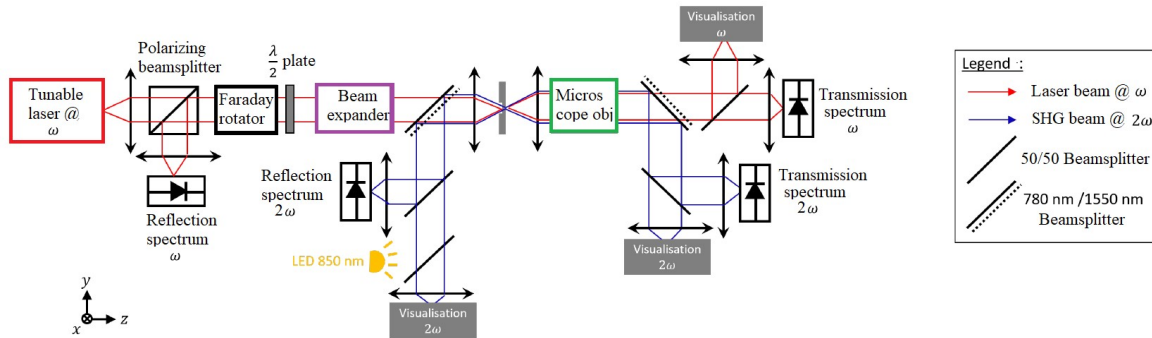
Figure 2. Characterization setup used to measure the pump and SHG signal response of the fabricated CRIGFs
