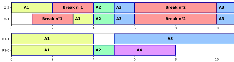
■ Figure 1 Operator and resource oriented Gantt chart for the example instance.
