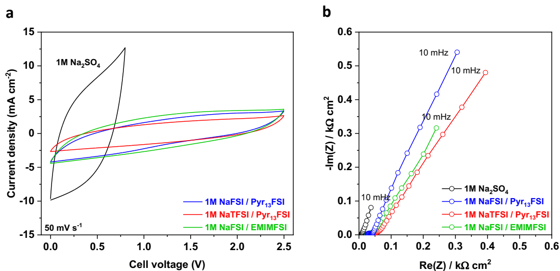
Figure S12. Electrochemical supercapacitor behaviour in Na salts-based ionic liquids using very thin film of Ni / MnO 2 electrodes (5 min Ni DHBT + 1000 cycles of MnO 2 ). a) Cyclic voltammogram recorded at 50 mV s -1 up to 2.5 V. b) EIS characteristics from 100 kHz to 10 mHz.
