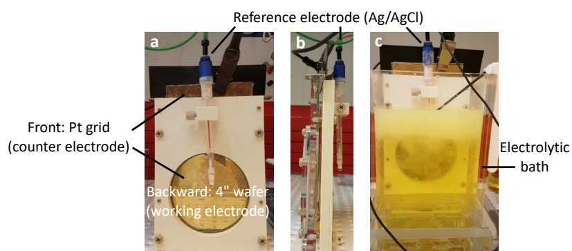
Figure S9. Electrochemical cell dedicated for 4-inch substrates for large-scale electrolytic deposition of the porous current collector and active material. a) Front view. b) Side view. c) Immersed in the deposition bath. The custom-made cell was designed in collaboration with Yamamoto-MS.
