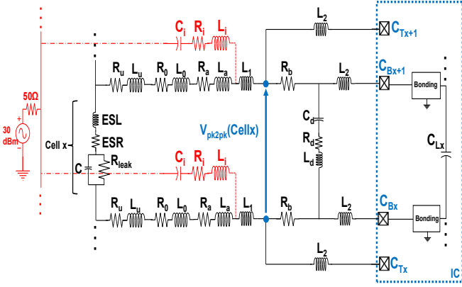
Fig. 8. Proposed BMS IC architecture for maximizing the cell balancing impact on injection levels.
