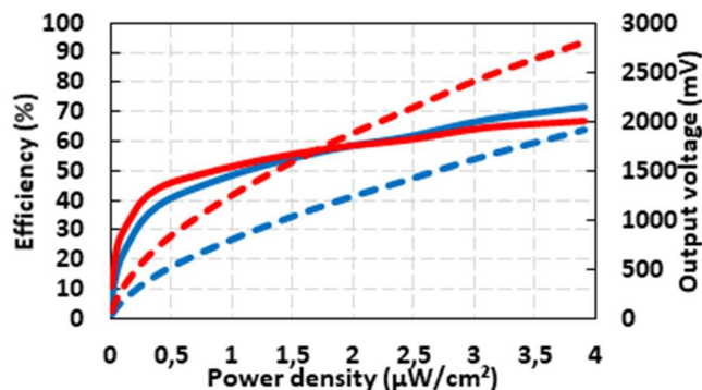
Fig. 9. Computed efficiency (full lines) and measured output DC voltage (dashed lines) against power densities for the printed folded quart-wavelength dipole rectenna with capacitive arms without (blue) and with (red) the use of a 6 cm x 8 cm reflector plane located at 5 cm below the antenna/rectenna, at 868 MHz and for a 10 k \Omega resistive load.
