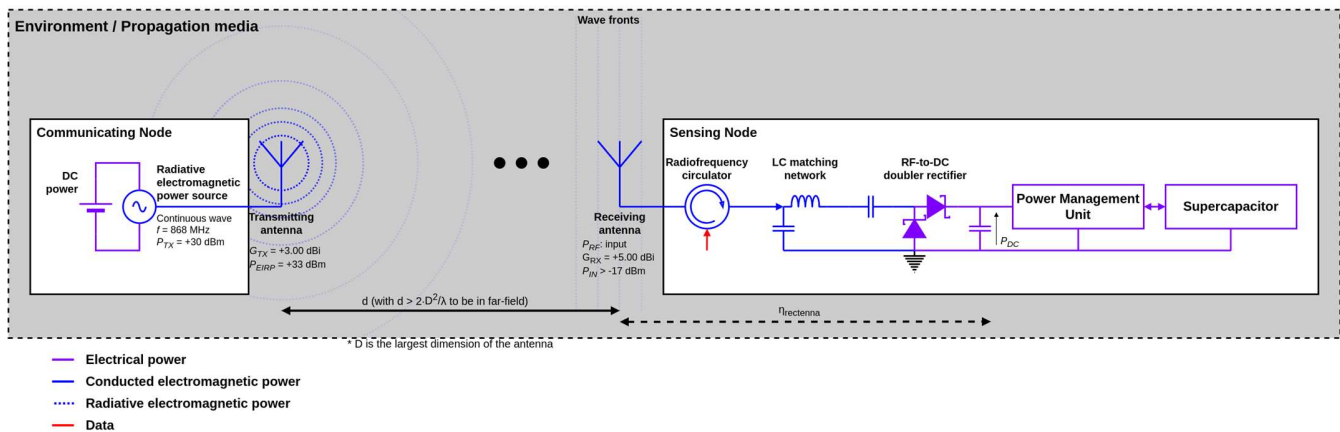
Fig. 5. Bloc diagram of the implementation of the Wireless Power Transfer solution.
