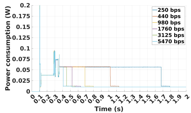
Fig. 13. Power consumption of the Sensing Node against the data-rate, for a +4 dBm transmission power and a 4 bytes data payload.
