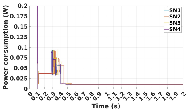
Fig. 17. Power consumption of the Sensing Nodes for a transmission power of +4 dBm and the fastest data-rate (DR5).
