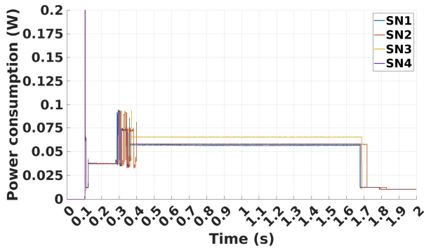
Fig. 16. Power consumption of the Sensing Nodes for a transmission power of +14 dBm and the slowest data-rate (DR0).
