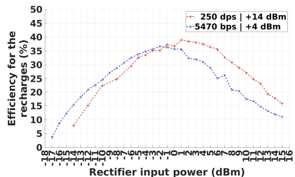
Fig. 19. Energy efficiency of the Sensing Nodes during the recharge against the conducted electromagnetic input power applied at the input of the rectifier, for a frequency of 868 MHz, and for two configurations of the wireless communication: transmission power of +4 dBm and data-rate of 5470 bps (blue), and transmission power of +14 dBm and data-rate of 250 bps (red).
