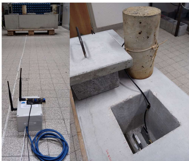
Fig. 20. Photographs of a complete Cyber-Physical System composed of 3 Sensing Nodes embedded in a reinforced concrete beam, and of 1 Communicating Node.
