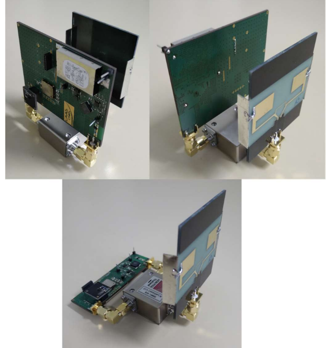
Fig. 11. Photographs of prototypes of the sensing nodes, using or not the Printed Circuit Board as a 6 cm x 8 cm metallic reflector plane located at 5 cm below the unique antenna.
