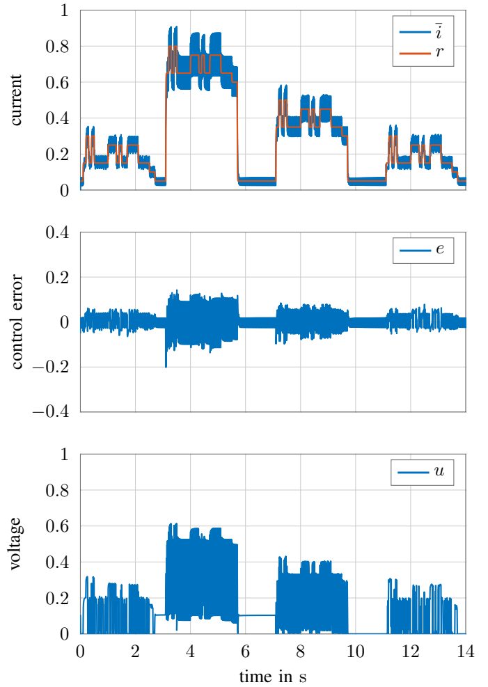
Fig. 5: Experimental results of the sliding mode controller for solenoid B. The values are normalized to i_A and v_{\text{bat}} , respectively.
