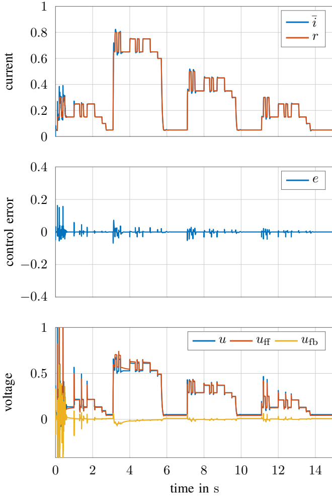
Fig. 12: Control signals of the indirect adaptive two-degrees-of-freedom control algorithm for solenoid C. The values are normalized to i_A and v_{\text{bat}} , respectively.
