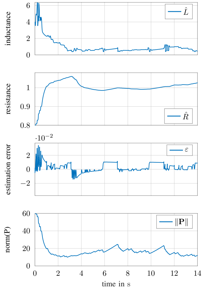
Fig. 13: Estimated parameters of the indirect adaptive two-degrees-of-freedom control algorithm for solenoid C. The values are normalized to L_C , R_C , and v_{\text{bat}} , respectively.
