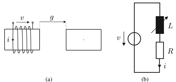
Fig. 1: Mechanical and electrical schematics of a solenoid.
