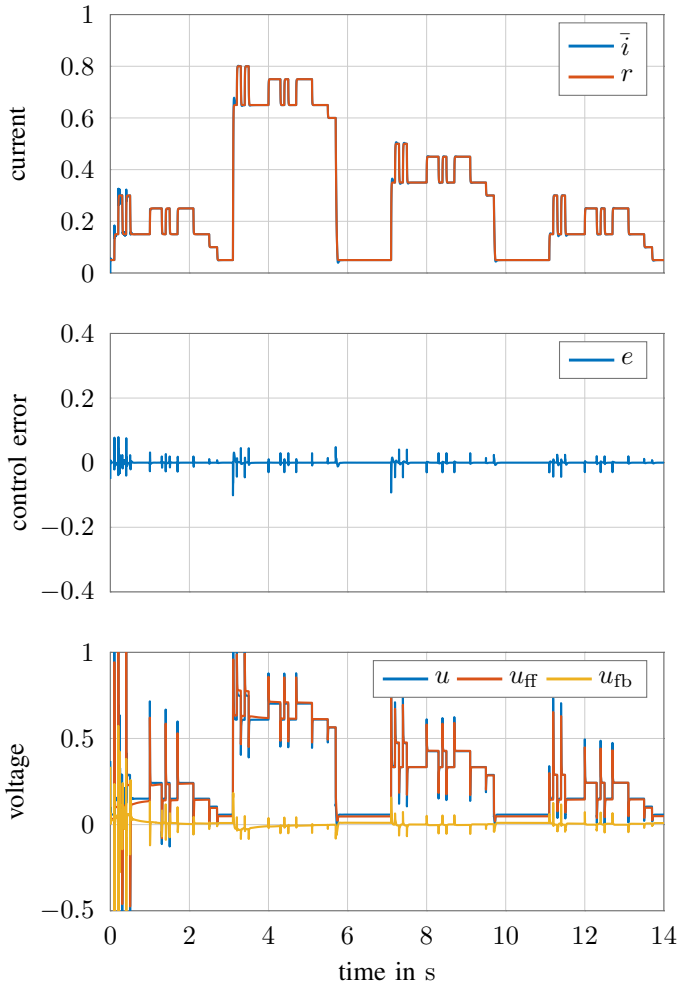
Fig. 8: Experimental results of the indirect adaptive two-degrees-of-freedom control algorithm for solenoid A. The values are normalized to i_A and v_{bat} , respectively.
