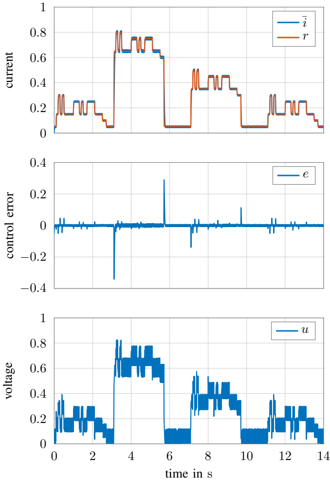
Fig. 4: Experimental results of the sliding mode controller for solenoid A. The values are normalized to i_A and v_{\text{bat}} , respectively.
