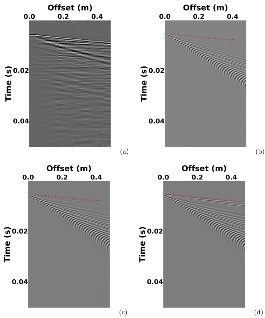
Fig. 10. Comparison between experimental filtered (a), 3D elastic (b), 2D elastic (c) and 2D poroelastic (d) seismicograms (vertical component of particle velocity) in the Full PMLs case.
