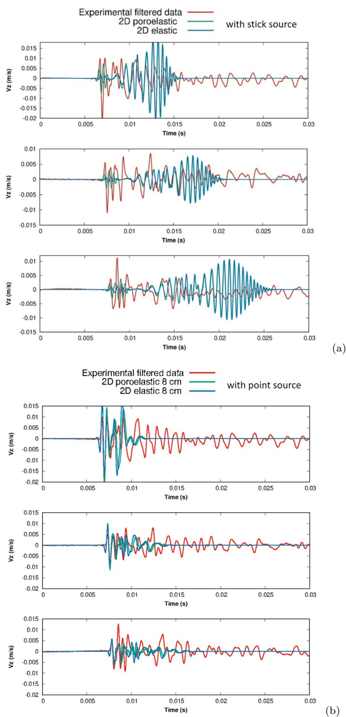
Fig. 19. (a) Comparison of the numerical seismograms (for the 2D elastic and 2D poro-elastic models) with the experimental filtered ones at receivers 10, 15, and 20 in the pure (original) stick case (time in seconds). (b) Same thing but in the 8 cm deep source case. All the seismograms are zoomed over the first 30 ms because there is no signal after 25 ms in the numerical seismograms due to the PML absorbing conditions.
