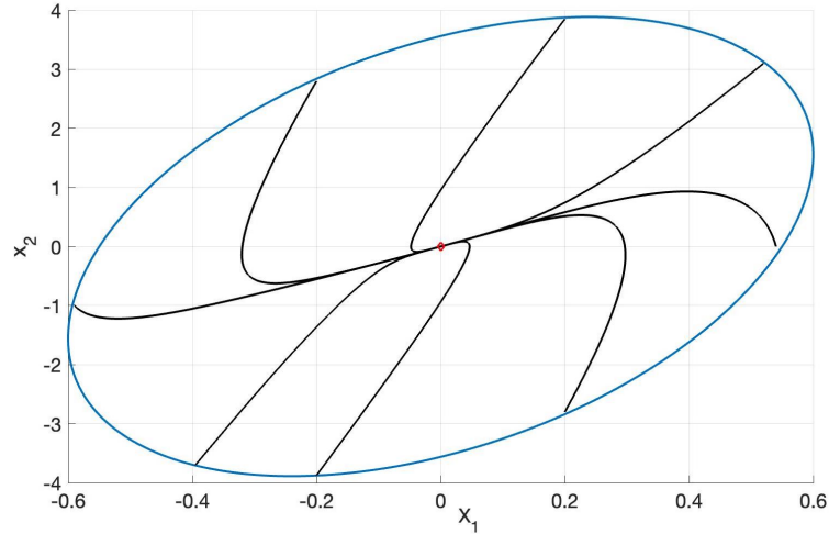
Figure 2: Trajectories of the closed-loop system with state-feedback (21)
