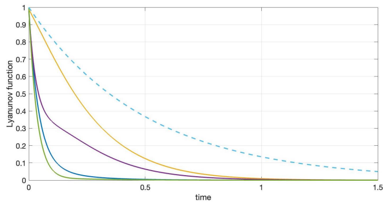
Figure 3: Lyapunov function along four trajectories with state-feedback (21)
