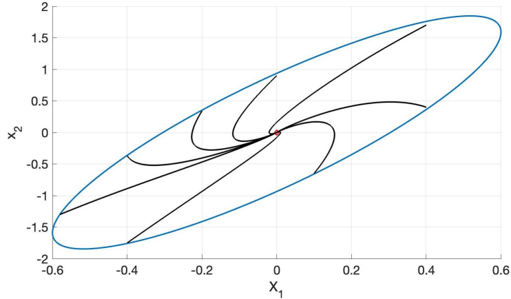
Figure 1: Trajectories of the closed-loop system with state-feedback (20)
