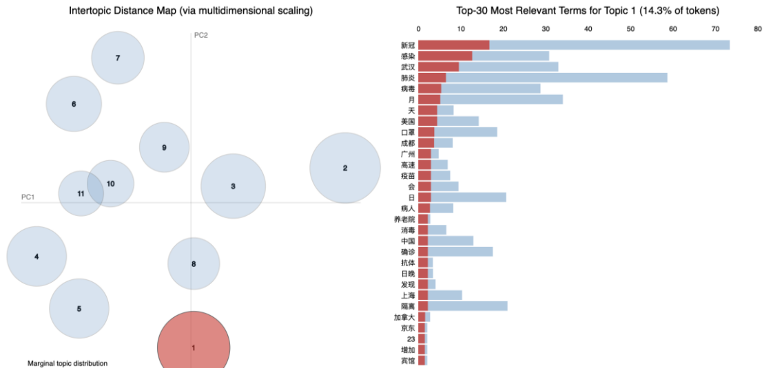
Figure 4. Visualization graph of LDA topic modeling for records classified into three groups
