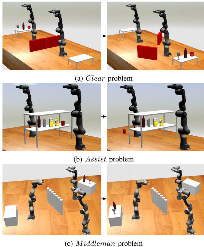
Fig. 1: A visualization of the initial and goal states of 3 of the multi-robot TAMP problems solved by our method.
