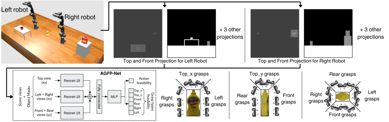
Fig. 2: Visualization of the feasibility prediction pipeline on an example 2-robot scene. (Top) Scene depth images are constructed for each robot such that only the objects in the workspace of the robot are shown. Objects present in both robots workspaces are visible in both scene projections (yellow mustard bottle). (bottom) Scene projections and object masks are given to AGFP-Net to obtain the action feasibility and the feasibility of 6 grasp types, illustrated on an example object.
