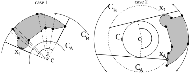
Figure 10: Relevant points considered by the algorithm
