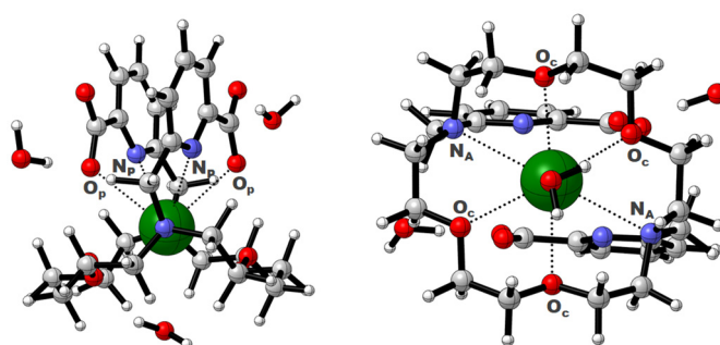
Fig. 3 Side and bottom views of the most stable conformation of [\text{Ra}(\text{macropa})(\text{H}_2\text{O})_3] at the SMD sr-MN15/ACVDZ level of theory. \text{N}_p = pyridyl nitrogen atoms, \text{O}_p = picolinate oxygen atoms, \text{O}_c = crown oxygen atoms, \text{N}_A = amine nitrogen.
