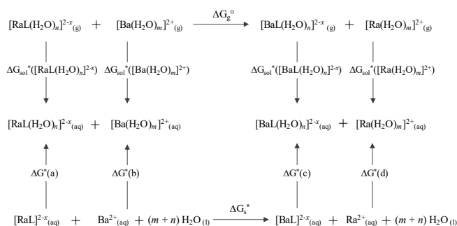
Scheme 2 Hess cycle used to calculate the Gibbs energy of the exchange reactions between Ra^{2+} and Ba^{2+} with explicitly treated solvent molecules.
