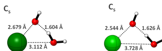
Fig. 2 Computed structure at the SMD sr-MN15/ACVDZ level of theory for the most stable conformation of [\text{RaOH}(\text{H}_2\text{O})_2]^+ (left) and [\text{BaOH}(\text{H}_2\text{O})_2]^+ (right).
