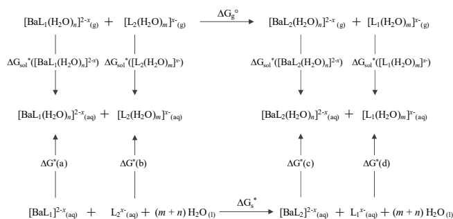
Scheme 1 Hess cycle used to calculate the Gibbs energy of the reaction (5) with explicitly treated solvent molecules.
