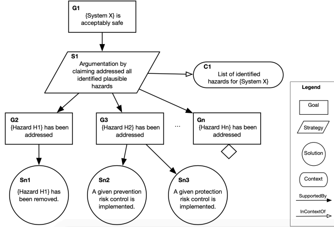
Figure 1: GSN example adapted from Hazard Avoidance Pattern [19]
