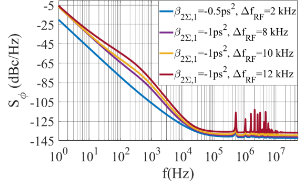
Fig. 4. Simulated phase noise evolution with detuning ( \Delta f_{RF} ) and for two intra-cavity chromatic dispersions: \beta_{2\Sigma,1} = (-0.5, -1) ps^2 under gaussian filter assumption.
