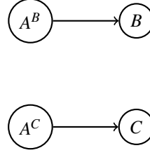
Figure 4: New simplified precedence graph with predecessor partition split.
