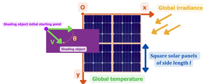
Figure 13. An illustration of the method to simulate the evolution of the P-V of the PV string under VPSC.
