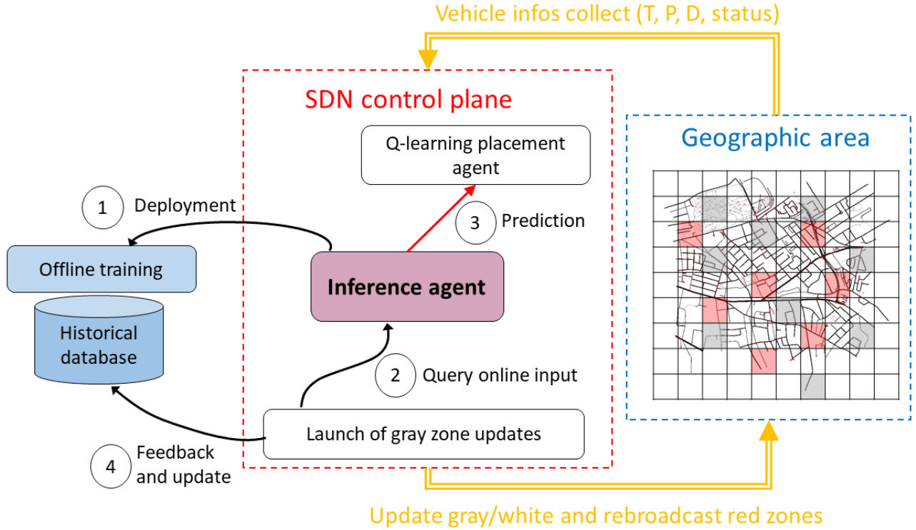
Fig. 4: Packet Reception Ratio (PRR) inference framework.
