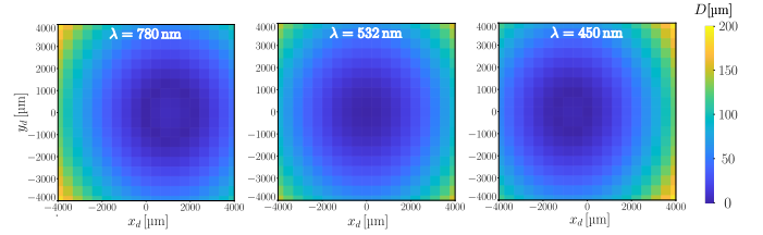
Fig. 9. Distance maps comparing the classical M_c model to Zemax for (left) upper, (centre) central and (right) lower wavelengths.
