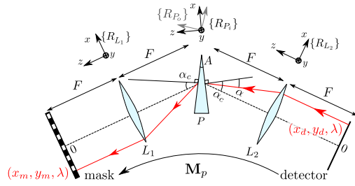
Fig. 5. The backward propagation model M_p is the combination of the elementary transformations l_{p,a} , p_{a,a} and l_{a,p} and the rotation operators R_{L_2 \rightarrow P_i} and R_{P_o \rightarrow L_1} .
