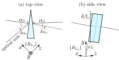
Fig. 6. Prism alignment parameters. The angle \alpha_c is the angle of incidence corresponding to the minimum deflection of the prism at the central wavelength. The angles \delta\alpha_c and \delta\beta_c describe small errors of alignment respectively with respect to the minimum deflection and with respect to the verticality of the prism.
