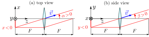
Fig. 2. Position-to-angle conversion l_{p,a} induced by a perfect thin lens between object and Fourier planes.
