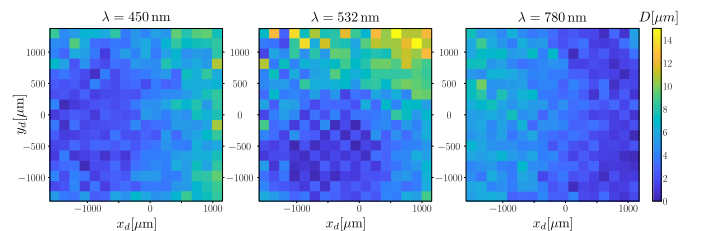
Fig. 16. Experimental reprojection error D for the 3 reference wavelengths.
