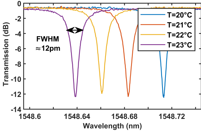
Fig. 8: Optical transmission spectrum of MRR with 120 \mu\text{m} radius measured with APEX206 OSA at different temperatures.
