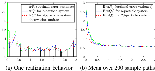
Fig. 2: Evolution of the second moment of the continuous-discrete optimal filter and particle filter.
