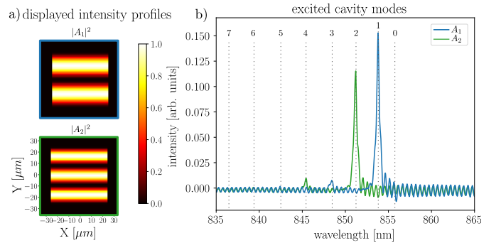
Fig. 3. Selective excitation of the high-order cavity modes along the y direction.
