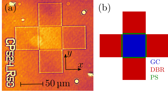
Fig. 1. (a) Top view of the 2D CRIGF under study; (b) Schematic of the 2D CRIGF with a 2D central grating coupler (GC), surrounded by four phase sections (PS) and four distributed Bragg Reflectors (DBR). Incident light coupled by the GC is trapped in the 2D Fabry-Pérot cavity formed by the DBRs.
