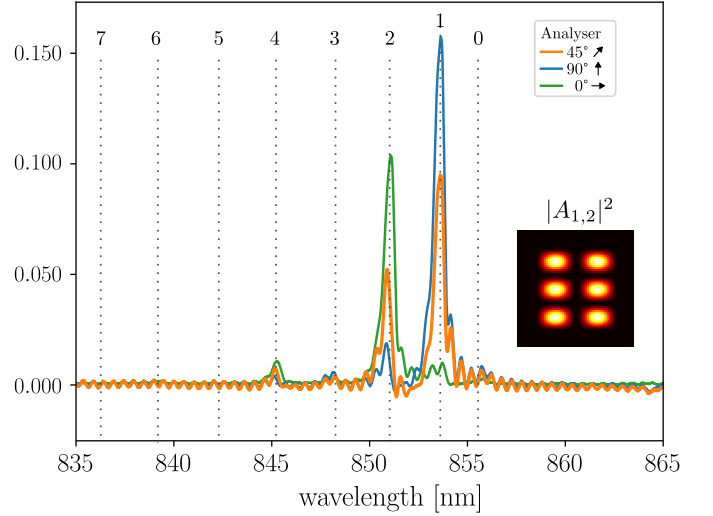
Fig. 6. Selective excitation of the 2D cavity with asymmetric 2D shaped beams, polarized at 45^\circ , for different orientation of the analyser placed before the photodiode collecting the reflected light.
