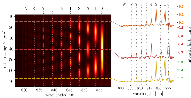
Fig. 2. Spatio-spectral map of reflectivity exhibiting the higher-order radiative patterns of the cavity along the y direction. The vertical dashed lines correspond to the wavelengths of the corresponding modes.
