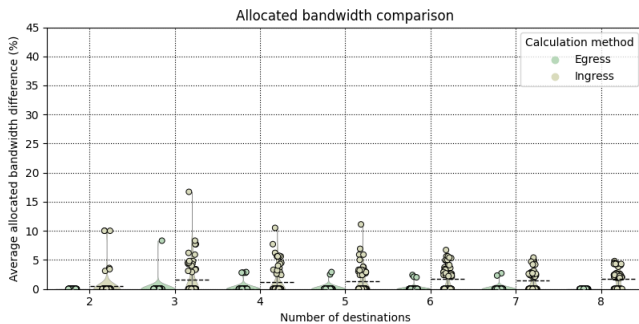
Figure 13: Allocation comparison (25% domains with P2M)
