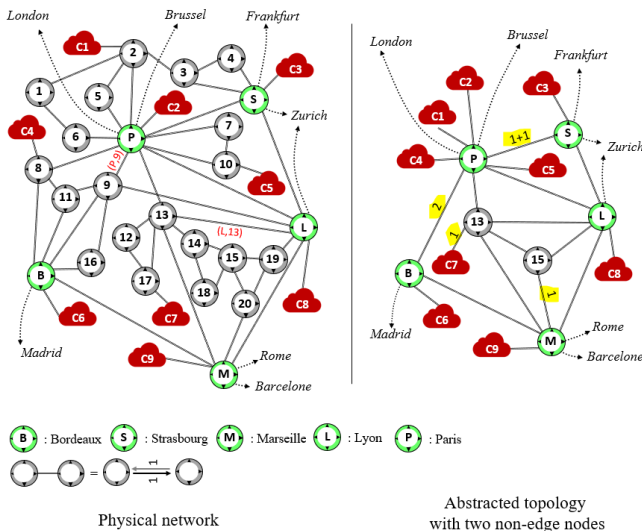
Figure 9: Physical & aggregated French network
