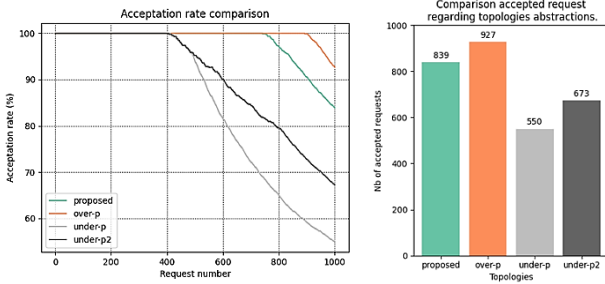
Figure 11: Demand acceptance for different aggregated topologies, with demands from the French
