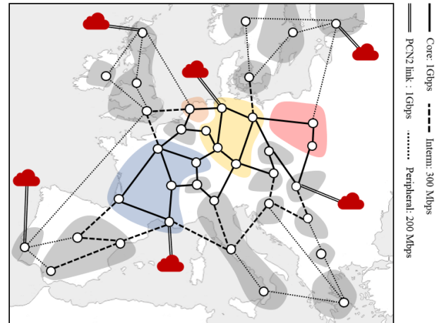
Figure 7: COST 266 based multi-domain network
