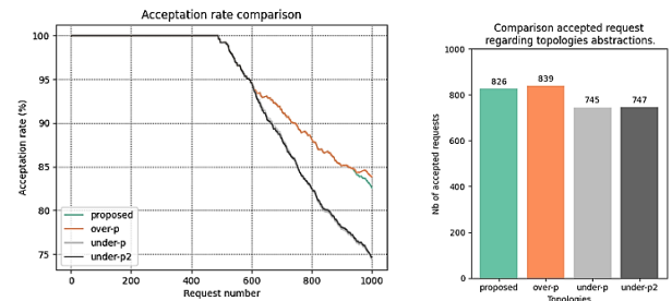
Figure 10: Service demand acceptance comparison for different Polish & French aggregated topologies
