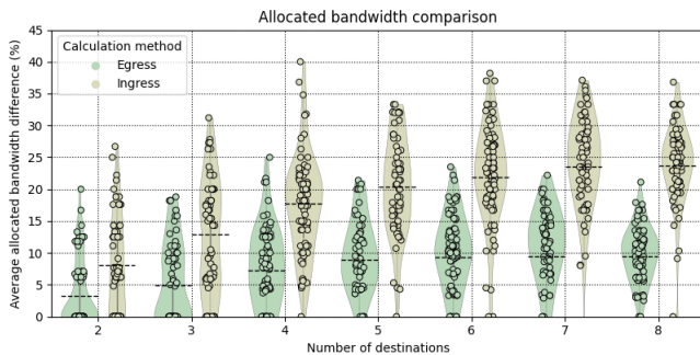
Figure 12: Allocation comparison (75% domains with P2M)
