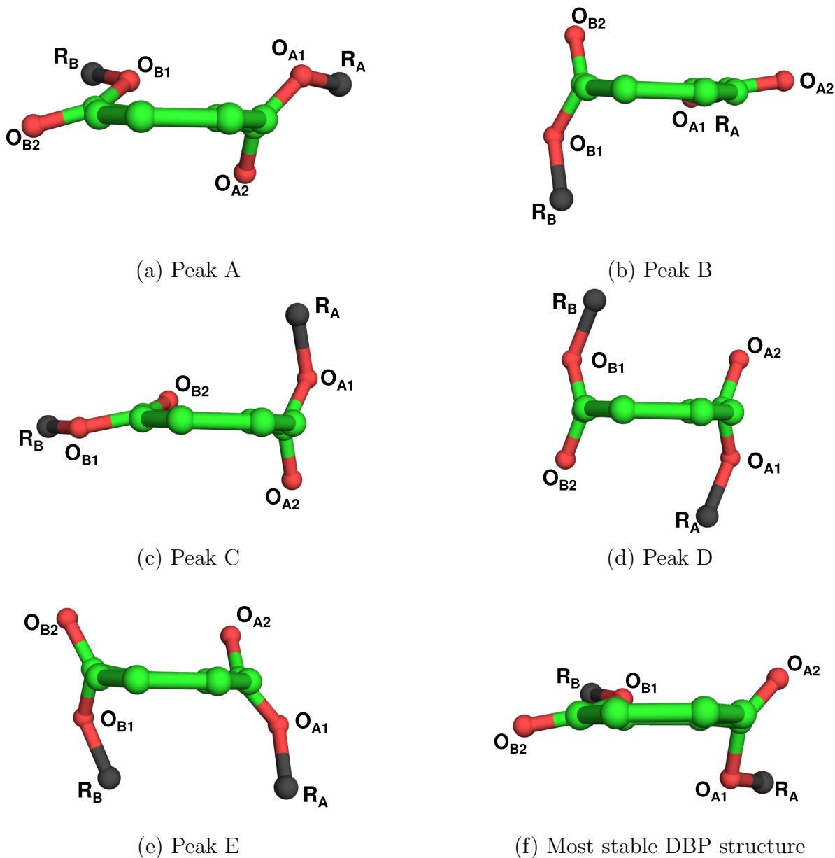
Figure 7: Illustration of the ester groups relative orientation for characteristics structures of the DBP excitation spectrum main peaks (Fig. 4-(a)).
