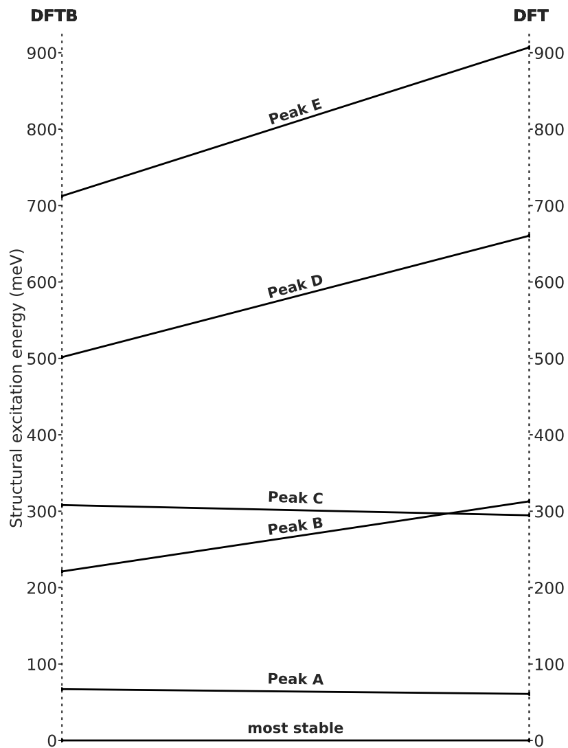
Figure S8: Comparison of DFT and DFTB energies of the characteristic DBP structures of the main peaks: lines connect the DFTB (left) and DFT (right) structural excitation energies (in meV) of the main peaks structures identified in figure 4. The DFTB(resp. DFT) structural excitation energy reference correspond to the lowest-energy structure computed at the DFTB(resp. DFT) level.
