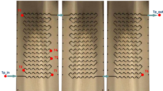
Fig. 2. The process channel and the positions of inner thermocouples
