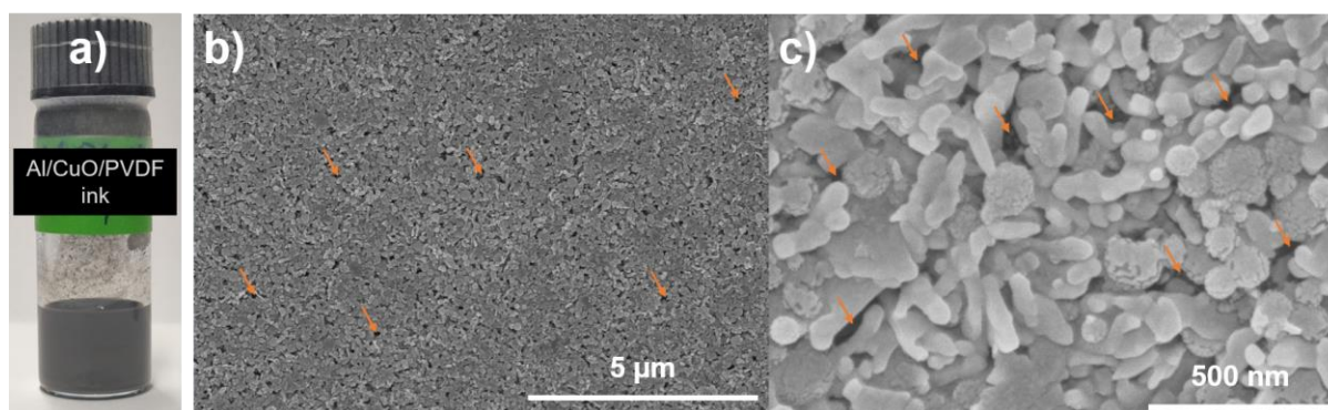
Figure 5. Optical (a) and SEM (b-c) image of the Al/CuO/PVDF ink. The orange arrows indicate mark the location of the micro-pores.
