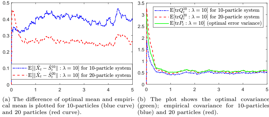
Figure 2: Comparison of mean and covariance for the optimal and ensemble filters with mean sampling rate \lambda = 10 .
