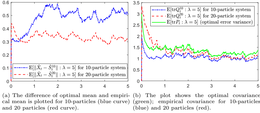
Figure 1: Comparison of mean and covariance for the optimal and ensemble filters with mean sampling rate \lambda = 5 .
