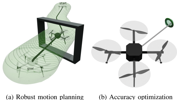
Fig. 1: Two scenarios considered for the experimental validation of the proposed method: (a) Robust navigation of a drone through a narrow window. (b) Precision in-flight ‘ring catching’ task, where the uncertainty on the position of the perch end-effector is minimized to successfully accomplish the task. A video of the experiments is available at: https://laas.hal.science/hal-04642257
