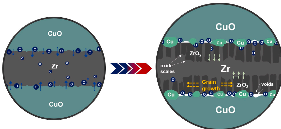
Fig. 9. A simplified schematic depicting the microstructural evolution of the Zr layer. The oxidation process, facilitated by outward oxygen migration, leads to the formation of columnar structures within the Zr layer. Subsequent oxidation results in the expansion of these structures into larger grains.
