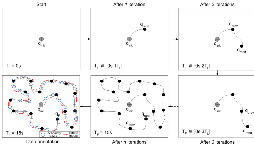
Figure 3: Dataset generation process. At each iteration, a new state \mathbf{q}_{rand} is randomly sampled from a uniform distribution and connected to the previous connected state \mathbf{q}_{prev} using a steering method. If the local trajectory (between \mathbf{q}_{rand} and \mathbf{q}_{prev} ) execution time is greater than 1s, it is truncated to 1s. Similarly, when the total trajectory time ( T_F ) exceeds 15s after adding a new state, we truncate at 15s. After n iterations, a trajectory with a total execution time of 15s made up of 1s sub-trajectories is generated. Finally, to annotate the data, the uncertainty tubes and control inputs are computed by simulating the tracking of the generated trajectory under nominal parameters (i.e \mathbf{p} = \mathbf{p}_c ).
