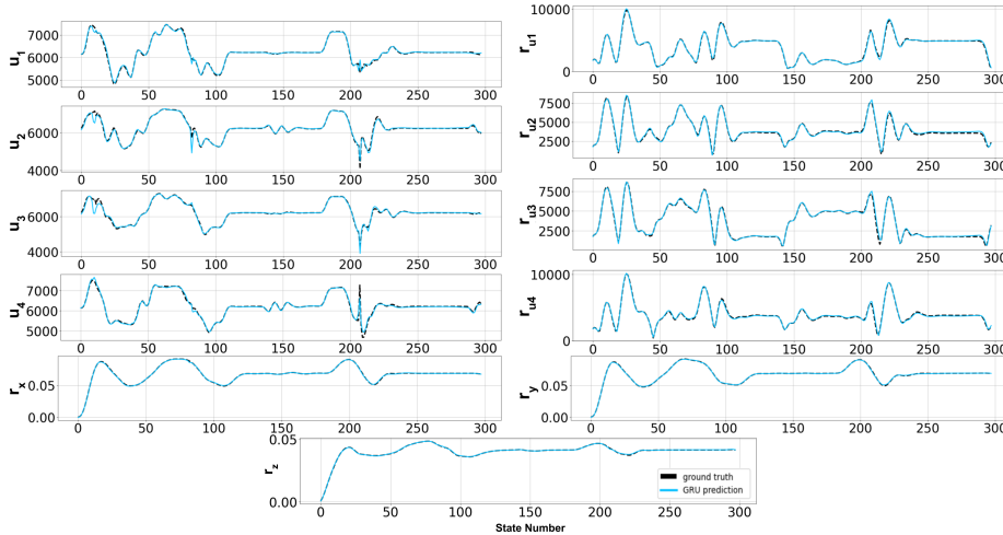
Figure 5: Example of GRU predictions on a 300-state trajectory of the test set. Predicted outputs are displayed in blue against true values in black. r_x, r_y, r_z are expressed in m , and control input associated values (u_i, r_{ui}) are squared propeller speeds [(\text{rad/s})^2] .
