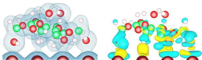
Fig. 5 Isosurfaces of the electronic density (isovalue 0.03 e/\text{\AA}^3 ) (left), and of the electronic density difference (isovalues +0.0018 e/\text{\AA}^3 in yellow and -0.0018 e/\text{\AA}^3 in cyan) (right), for the U- \Lambda -U orientation of the lactose molecule adsorbed on Cu(110).
