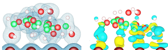
Fig. 5 Isosurfaces of the electronic density (isovalued 0.03 \text{ e}/\text{\AA}^3 ) (left), and of the electronic density difference (isovalues +0.0018 \text{ e}/\text{\AA}^3 in yellow and -0.0018 \text{ e}/\text{\AA}^3 in cyan) (right), for the U-Λ-U orientation of the lactose molecule adsorbed on Cu(110).
