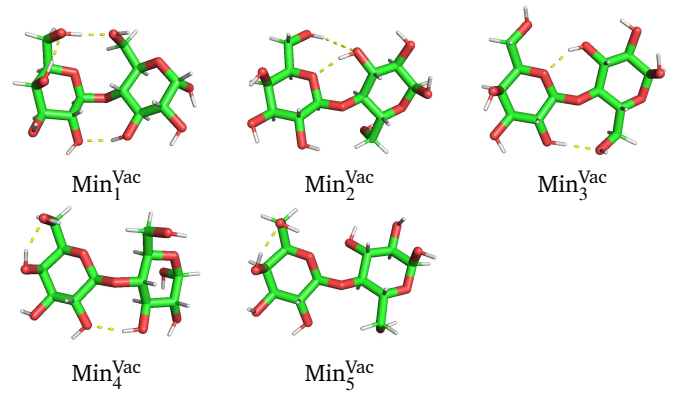
Fig. 2 The five low-energy vacuum conformations \text{Min}_{1,2,3,4,5}^{\text{Vac}} of \alpha -lactose localized by the IGLOO exploration and subsequently minimized using DFT. Carbon atoms are depicted in green, oxygen in red, hydrogen in white and H-bonds using yellow dashed lines.
