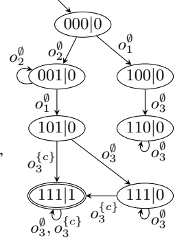
Figure 2: \Pi^{\mathcal{C}} = \langle \mathcal{V}^{\mathcal{C}}, \mathcal{O}^{\mathcal{C}}, I^{\mathcal{C}}, G^{\mathcal{C}} \rangle task constructed from the task \Pi from Fig. 1 and assuming we were able to infer the specified mutex. States in the reachable part of the state space of \Pi^{\mathcal{C}} are annotated with values of variables p, q, r, v_c in this order, e.g., the state \{\langle p, 1 \rangle, \langle q, 0 \rangle, \langle r, 1 \rangle, \langle v_c, 0 \rangle\} is annotated as 101|0.
