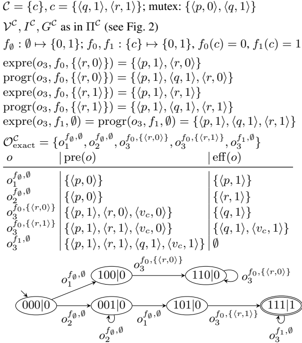
Figure 3: \Pi_{\text{exact}}^C = \langle \mathcal{V}^C, \mathcal{O}_{\text{exact}}^C, I^C, G^C \rangle task constructed from the task \Pi from Fig. 1 (assuming we were able to infer the specified mutex). States in the reachable part of the state space of \Pi_{\text{exact}}^C are annotated as in Fig. 2.
