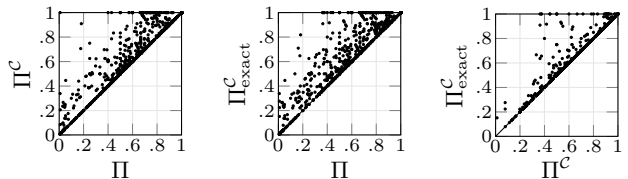
Figure 4: Comparison of h -values for initial states as ratios to the h^* -values for tasks where h^* -values are known. \Pi^C vs. \Pi_{exact}^C is compared over the same set of conjunctions inferred using \Pi_{exact}^C .
