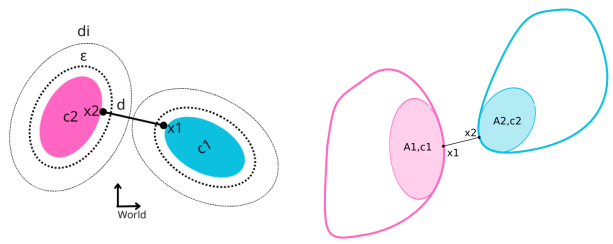
Fig. 3: Tangent ellipsoids at the closest points of two smooth collision geometries
