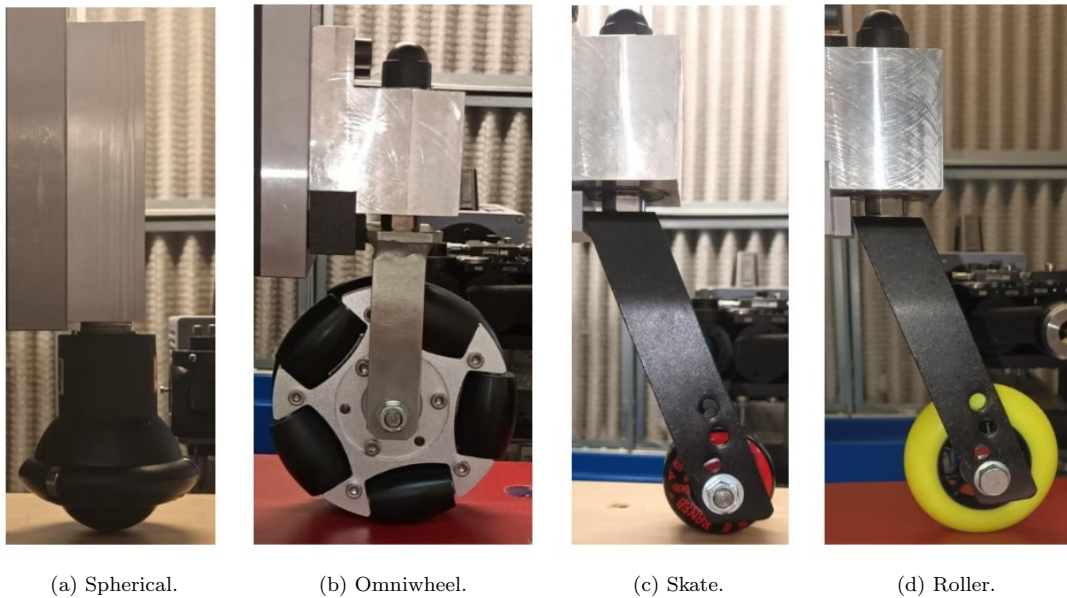
Figure 1. Caption. Casters tested in the study. The beige surface corresponds to the parquet and the red one to the Taraflex floor.
