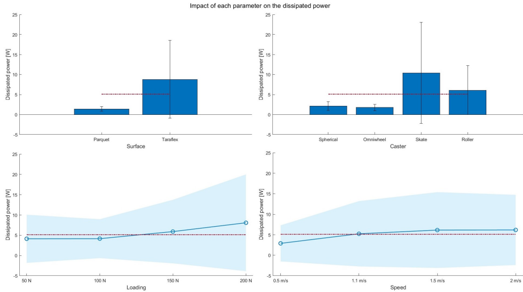
Figure 3. Impact of the parameters on the dissipated power for all the trials. The power values for each level of the parameter correspond to the average value of the power dissipated over all tests involving the level of the parameter concerned. The black error bars on the upper graphs and the colored areas on the lower graphs represent the standard deviation. The red line represents the mean value of the power dissipated over all the trials.
