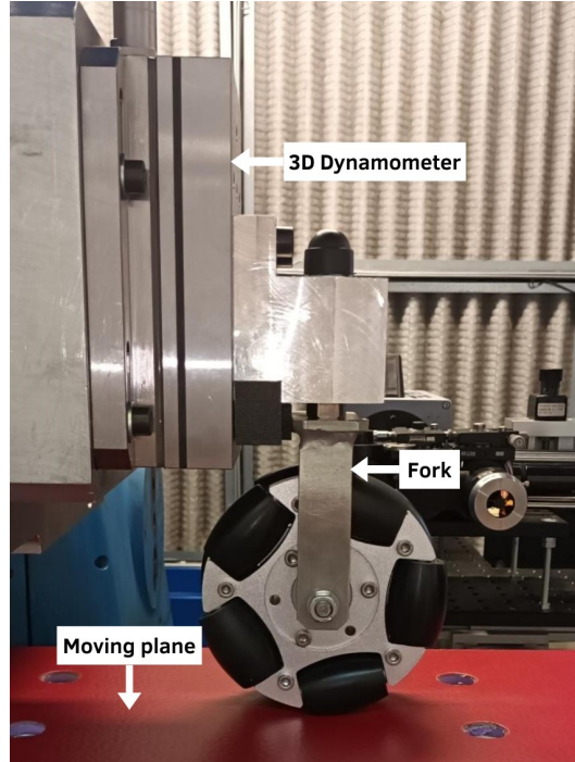
Figure 2. Caption. Test bench used for the study.
