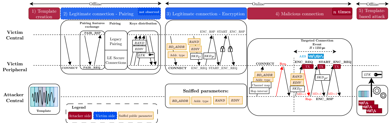
Figure 2. Attack overview.
