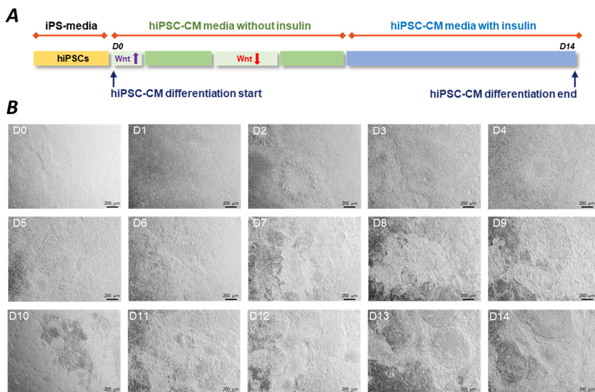
Figure 1. The process of hiPSC-CM differentiation. (A) Conventional cardiac differentiation protocols use CHIR99021 and IWP-2 or IWR-1 small molecules to sequentially activate and inhibit the Wnt/ \beta -catenin pathway, respectively. This panel shows a representative example of a typically applied hiPSC-CM differentiation protocol. (B) Representative images show the process of cardiac induction from Day 1 hiPSCs (D1) to Day 14 (D14) beating hiPSC-CMs. Small molecules were applied to a confluent hiPSC culture on D0. Cardiomyocytes showed spontaneous beating from D7. At D14, harvesting of the hiPSC-CMs is followed by functional readouts and cryopreservation. Images were taken on hiPSC-CMs generated by BioTalentum Ltd., at 4 \times magnification; scale bar, 200 \mu m.
