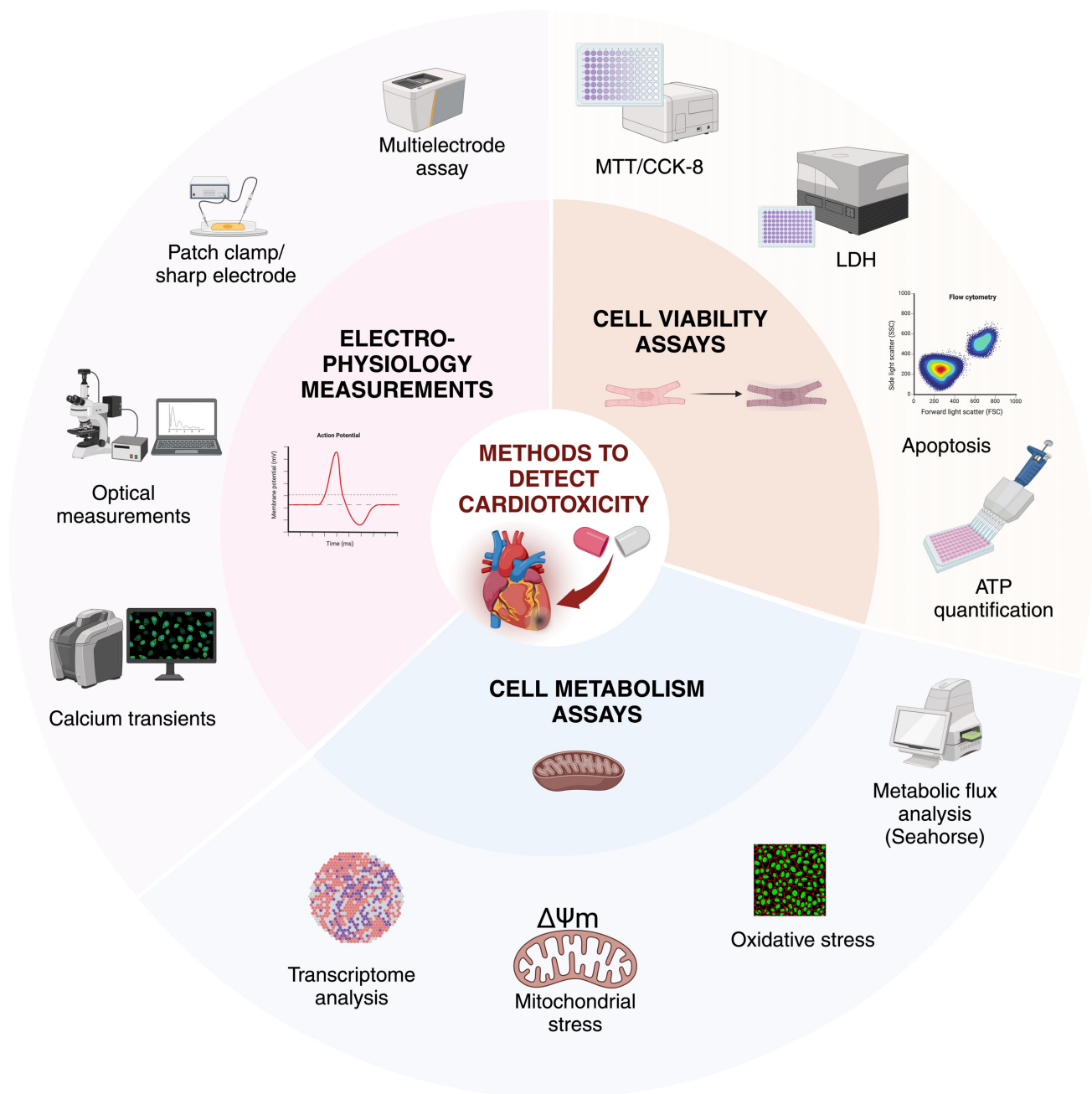
Figure 5. Methods to detect cardiotoxicity in CMs. In vitro, cardiotoxicity can be evaluated by a range of methods, including cell viability assays, cell metabolism assays, and electrophysiological readouts. Ion channel profiles, AP characteristics, and electrophysiological properties can be analysed by patch clamp, sharp electrode, or multielectrode measurements, in parallel with calcium transient kinetics and parameters. Cell viability can be monitored by ATP-release-based techniques, intracellular lactate dehydrogenase (LDH) activity, colorimetric assays such as MTT and CCK-8, and detected by a plate reader or by measuring apoptotic events. To quantify cell metabolism, the assessment of glycolytic and oxidative metabolism can be measured by Seahorse assays along with oxidative stress by measuring the toxic levels of ROS. Mitochondrial stress tests provide information on the resting respiration of the cells, by determining ATP production and oxygen consumption. Transcriptomic analysis and metabolomics focus on the underlying genes and their expression, the end products of these genes, and on the possible interactions in the metabolic pathways. Created with BioRender.com.
