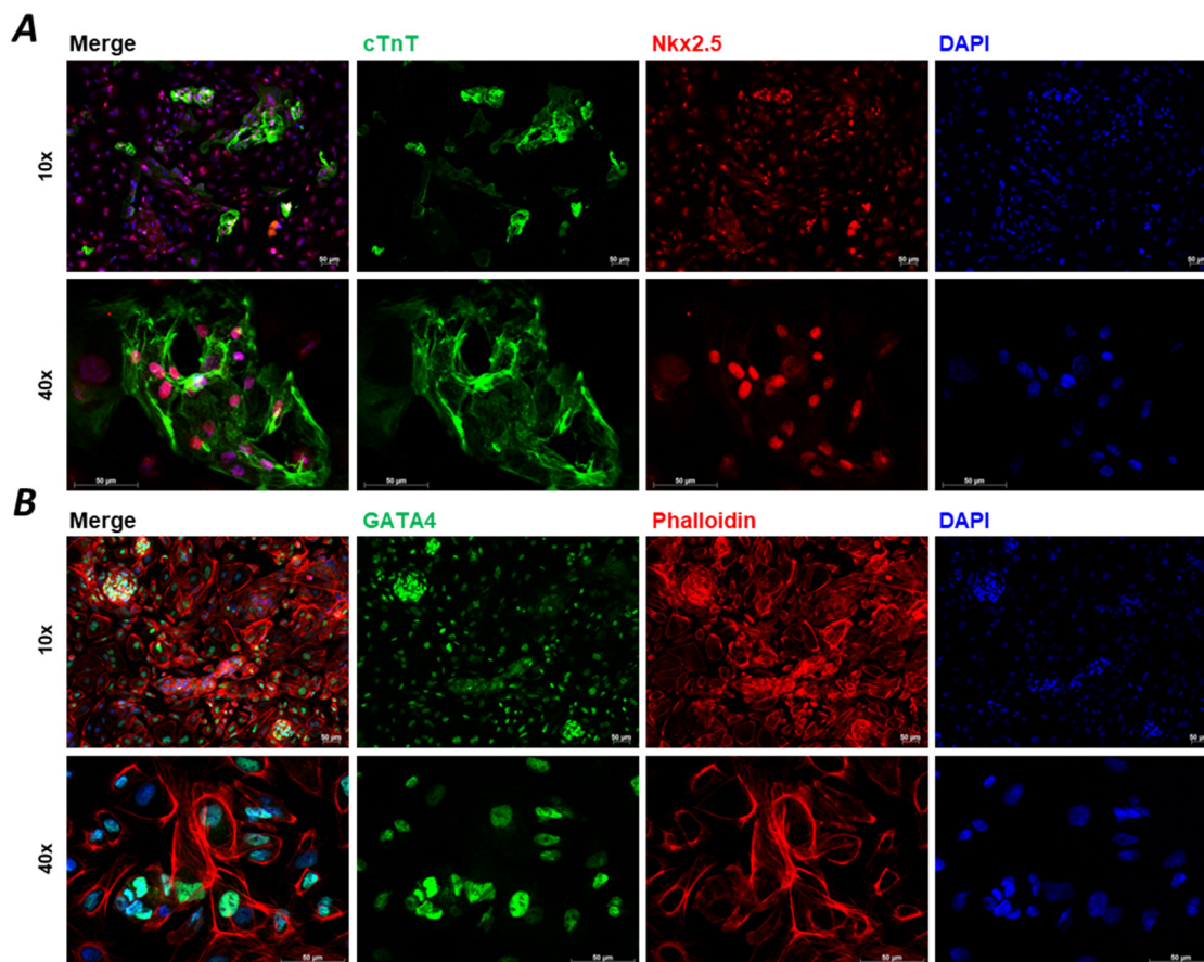
Figure 2. Immunocytochemistry staining of D15 2D hiPSC-CMs. Immunocytochemistry images of specific biomarkers for hiPSC-CM characterisation at Day 15 (D15). Cardiac troponin T (cTnT) is the most generally used marker for CMs, which shows apparent striations ((A), green) in the case of the development of CM sarcomere structures. Other biomarkers, such as mesodermal marker homeobox protein Nkx2.5 ((A), red), transcription factor GATA4 ((B), green), and phalloidin ((B), red) are shown, while 4',6-diamidino-2-phenylindole (DAPI) shows nuclear staining ((A,B), blue). Images were taken on hiPSC-CMs generated by BioTalentum Ltd., at 10× and 40× magnification; scale bar, 50 μm.
