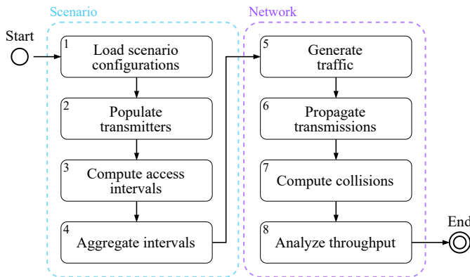
Fig. 7: Simulation workflow depicting the two-fold approach to the simulations: Scenario and Network.
