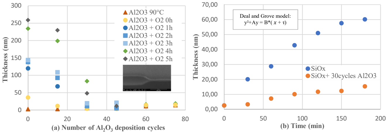
Figure 2. Ellipsometry measurements of (a) the dry thermal oxide thickness (with, as an inset, an SEM image of the oxide at an edge of an Al 2 O 3 covered area (right)) and (b) of the plasma-induced oxide.
