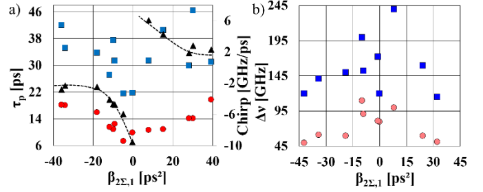
Fig. 8 a) Measurement with the stepped-heterodyne technique of the pulse FWHM (blue squares) and the instant frequency slope (black triangles) with the average optical cavity dispersion ( \beta_{2\Sigma,1} ). Calculated pulse FWHM at maximum of compression is given (red circle) through analytical chirp compensation applied to the experimentally measured pulses in order to simulate the impact of \beta_{2\Sigma,2} in a COEO. b) Experimental measurement of the spectral width at -10 \text{ dB} (red dots) and -50 \text{ dB} (blue square) from the main mode.
