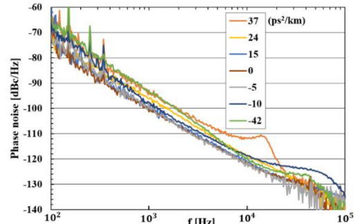
Fig. 9 Experimental phase noise measurement of the 10 GHz beat tone issued from the COEO for different \beta_{2\Sigma,1} ( \text{ps}^2 ) values (see legend). These phase noise curves were selected to show the global impact of the chromatic dispersion on the RF phase noise. The passive quality factor of the optical loop is also corrected here to an equivalent 400 m fiber spool COEO.
