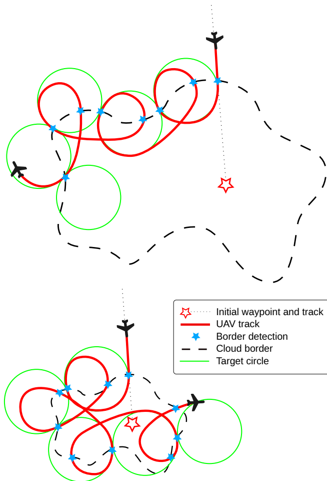
FIGURE 4: Resulting Trinity trajectory (in red) on a large cloud (top) and on a smaller one (bottom)
