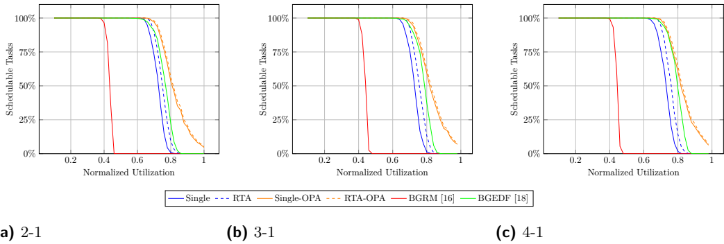
Figure 9 Schedulability ratios for m=2 processors and n=16 tasks.
