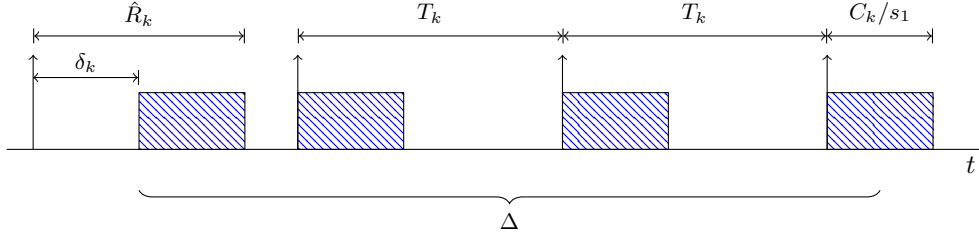
■ Figure 5 Sporadic task \tau_k maximum workload in generic time interval of length \Delta > 0 .
