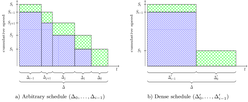
■ Figure 3 Two schedules from Theorem 6.
