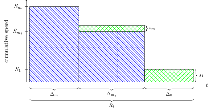
■ Figure 4 Execution of higher-priority jobs hp(i) (blue hatched) and job J_i ( i > m ) under analysis (green hatched) upon a two-speed multiprocessor (with m_1 fastest processors).
