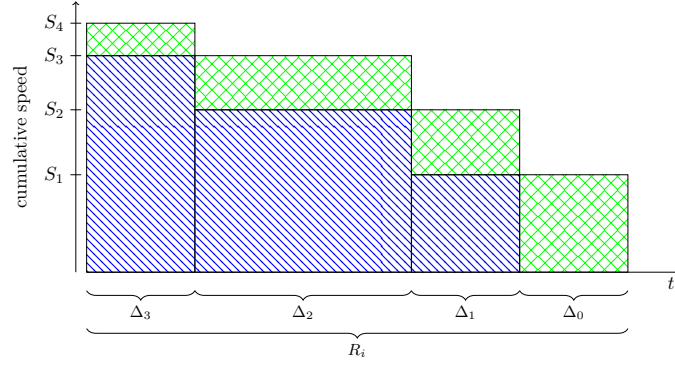
■ Figure 2 Execution of higher-priority jobs hp(i) (blue hatched) and job J_i under analysis (green cross-hatched).
