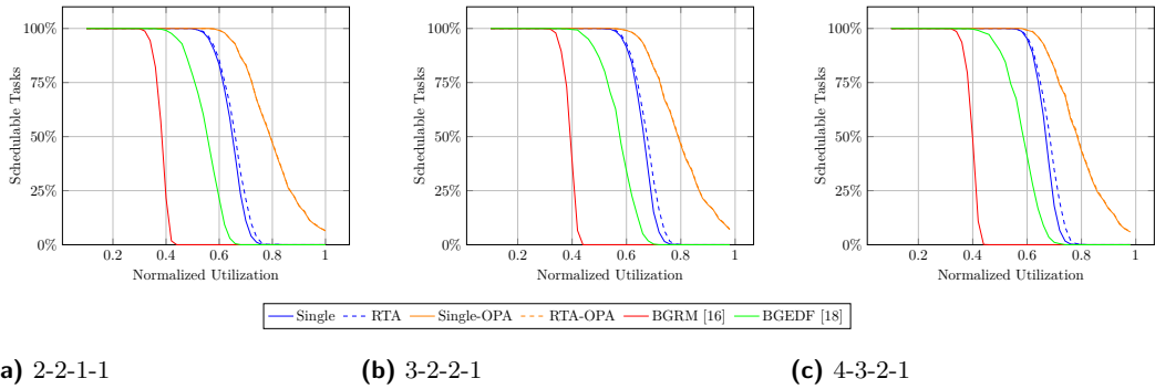
Figure 10 Schedulability ratios for m=4 processors and n=16 tasks.
