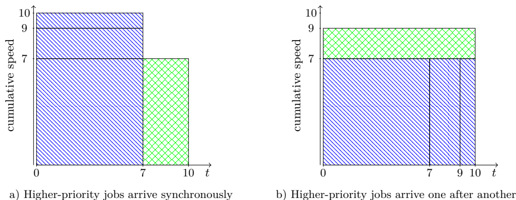
■ Figure 1 Fixed-priority schedules of four jobs on three processors ( m = 3 ) from Example 2.
